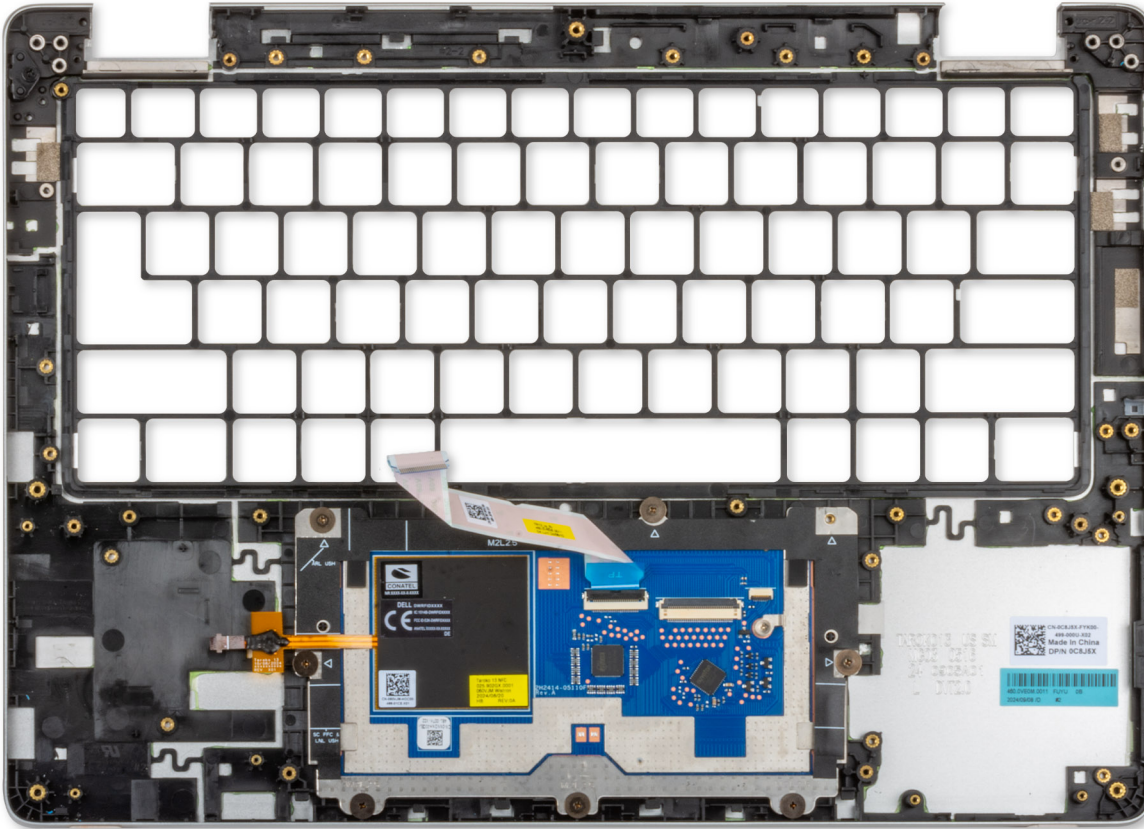
Figure 56. Removing the palm-rest assembly
