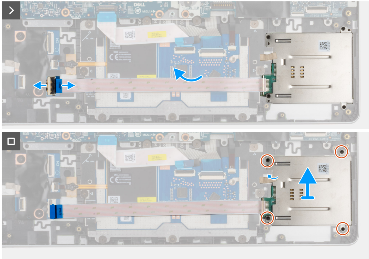
Figure 40. Removing the smart-card reader
