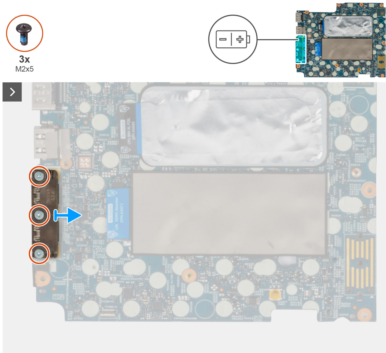
Figure 38. Removing the USB Type-C Connector Module
