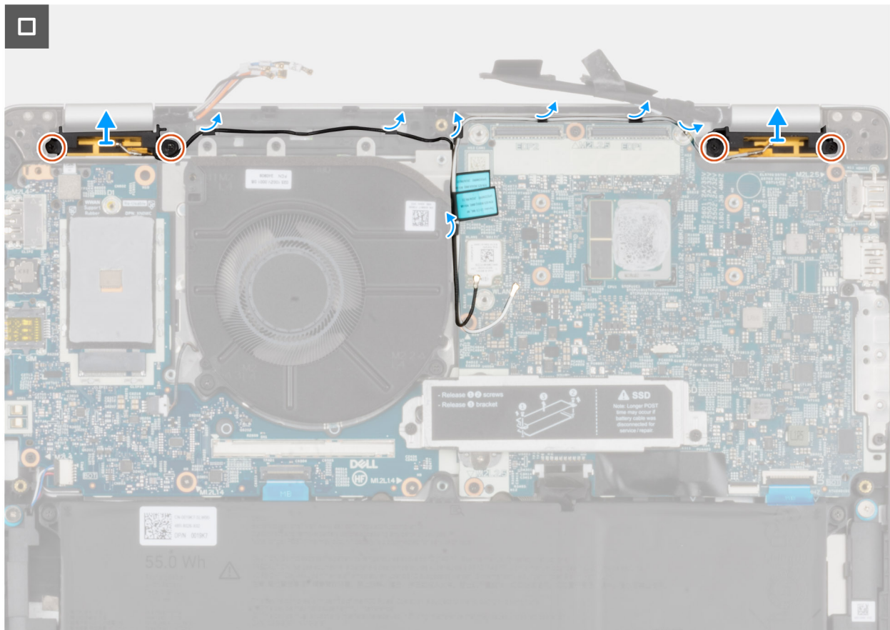
Figure 30. Removing the WLAN antenna module
