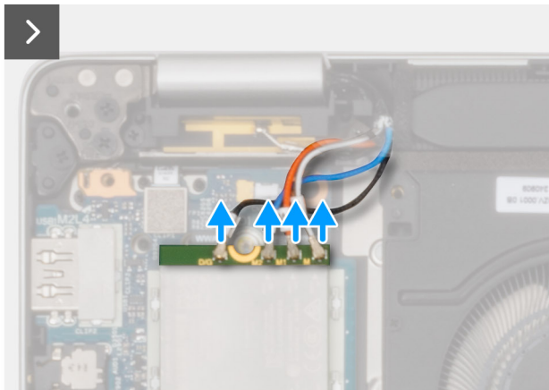
Figure 21. Removing the 5G WWAN card
