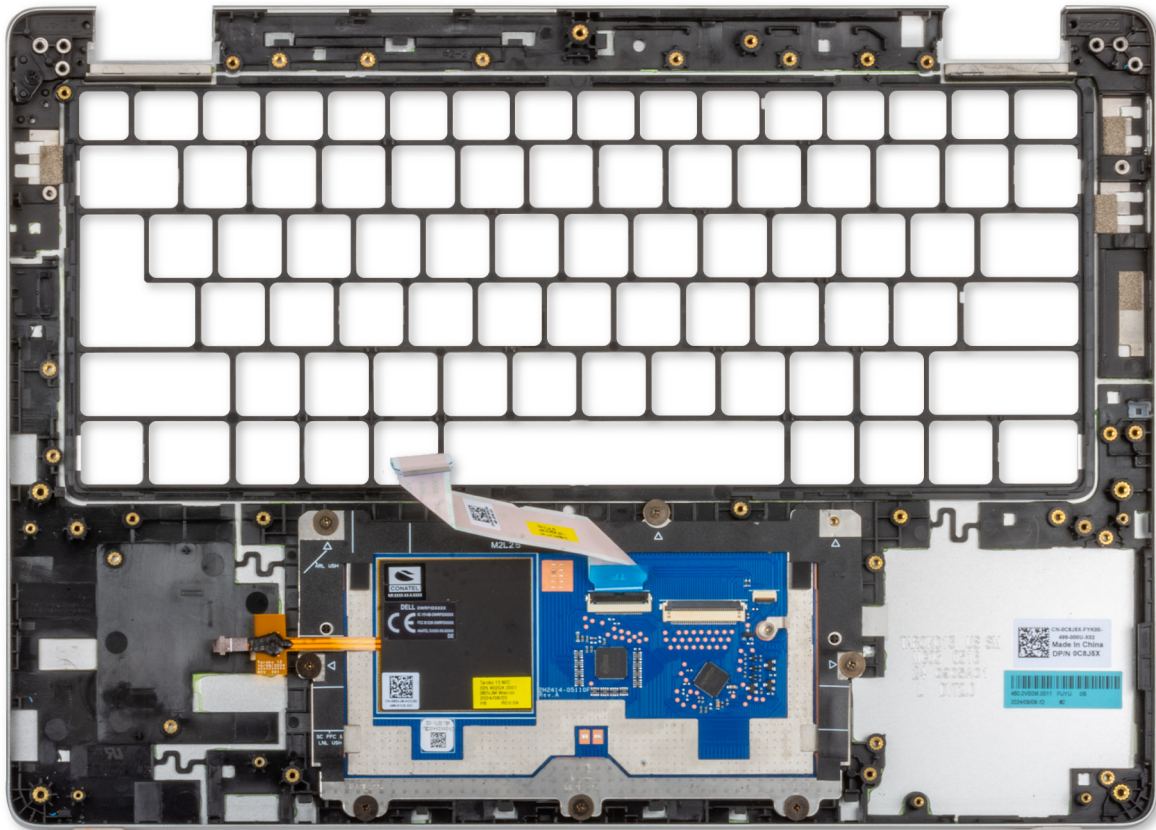
Figure 57. Installing the palm-rest assembly
