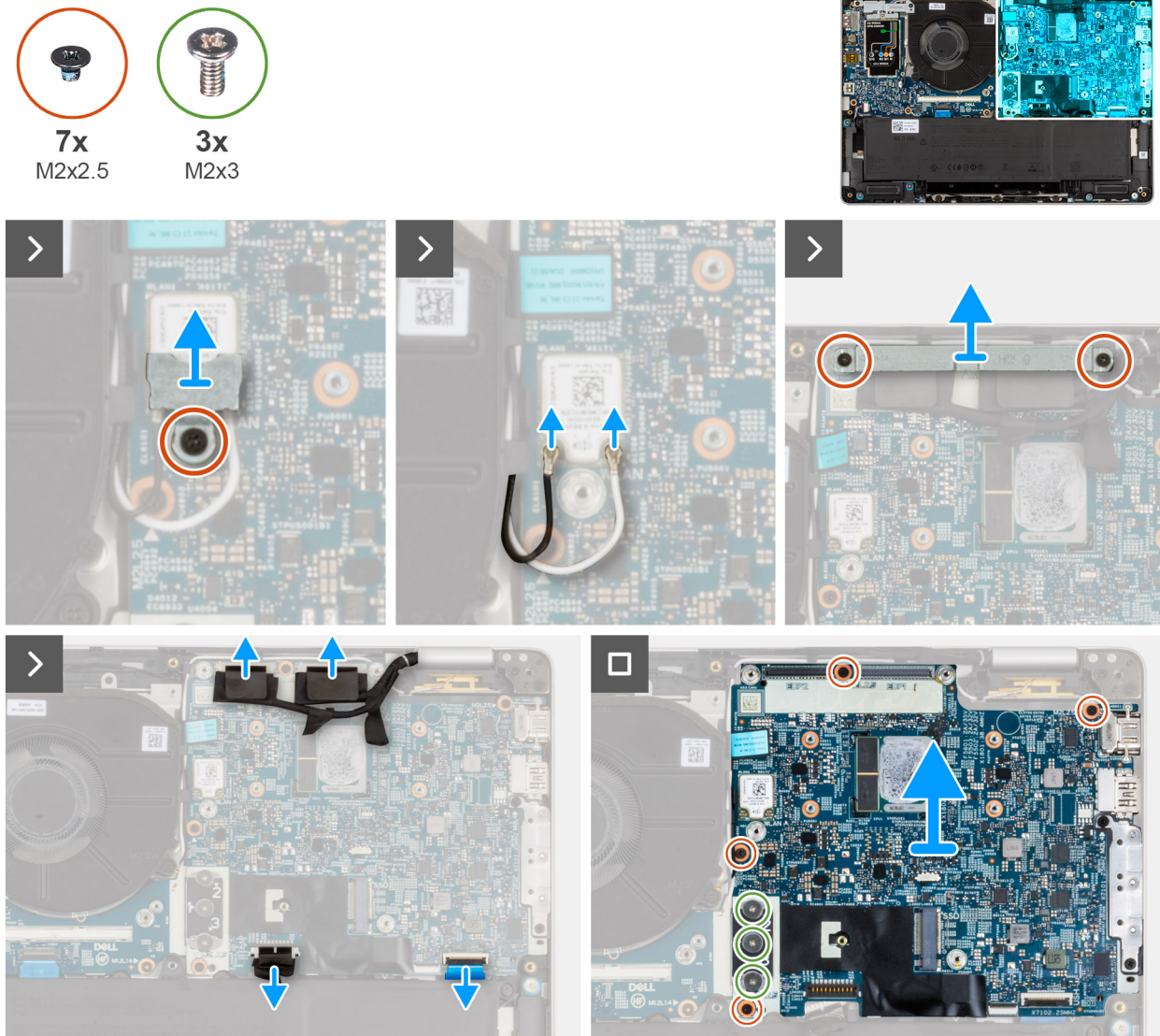
Figure 45. Removing the system board
