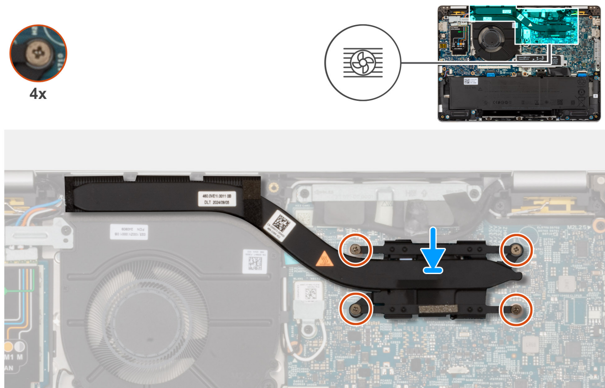
Figure 43. Installing the heat sink
