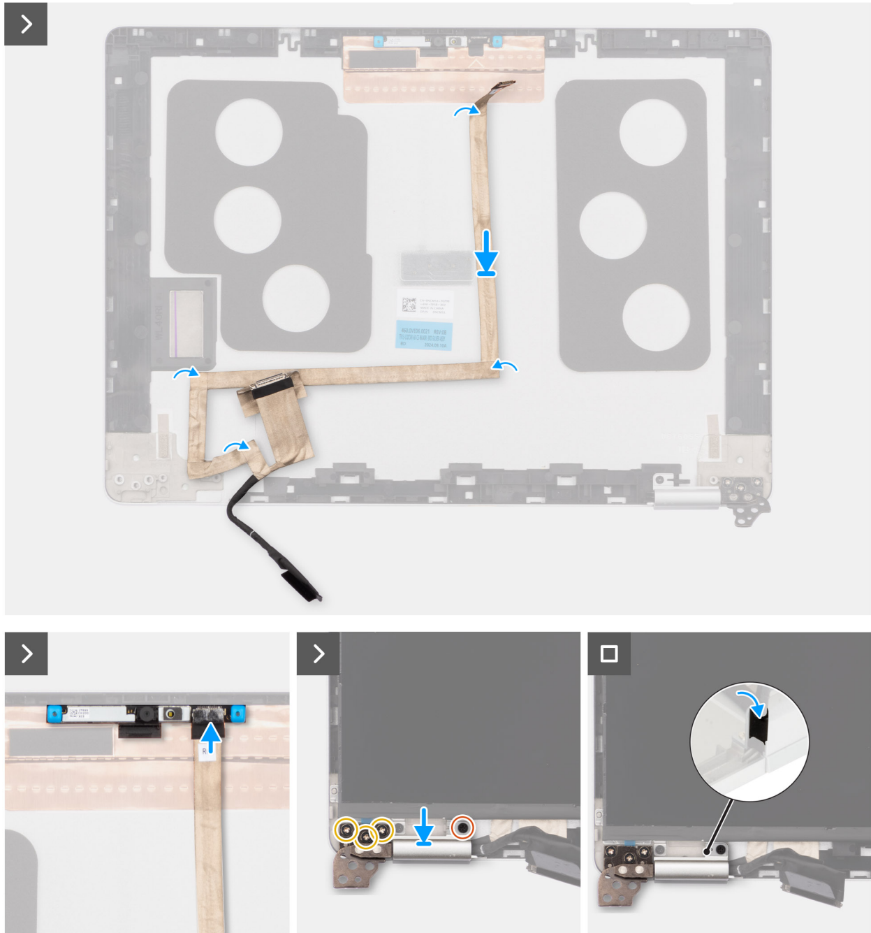
Figure 70. Installing the display cable
