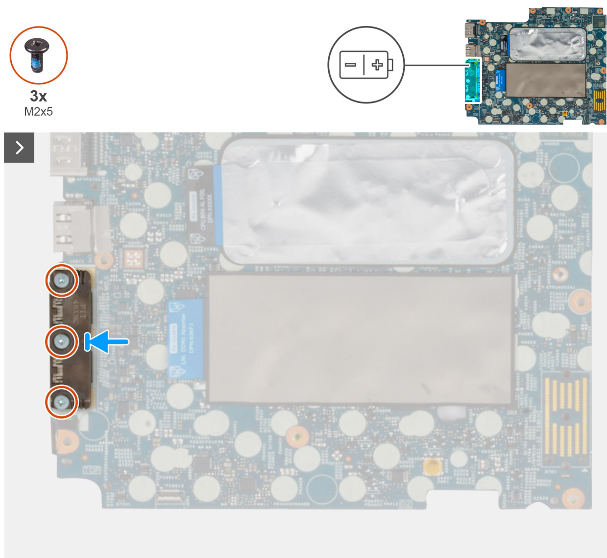
Figure 39. Installing the USB Type-C Connector Module
