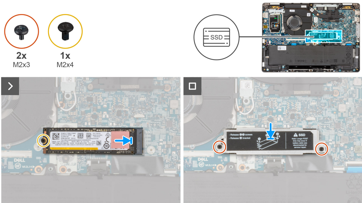
Figure 26. Installing the M.2 2280 SSD
