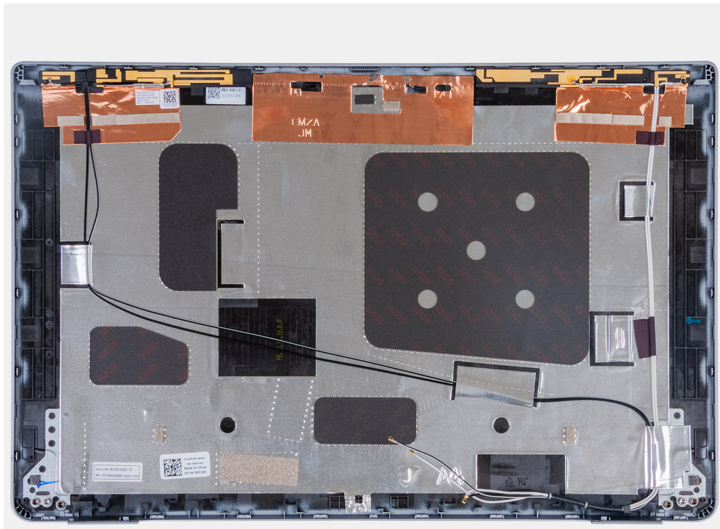
Figure 71. Removing the display back cover
