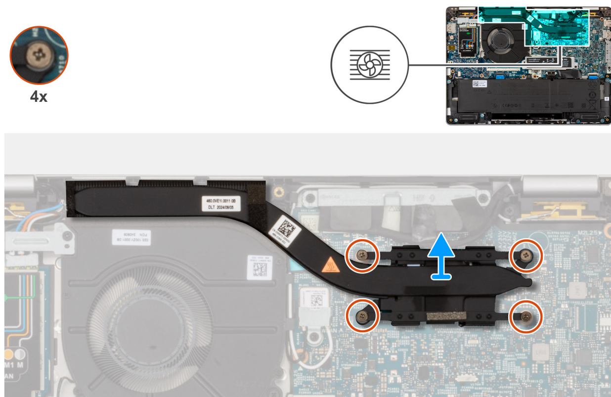
Figure 42. Removing the heat sink
