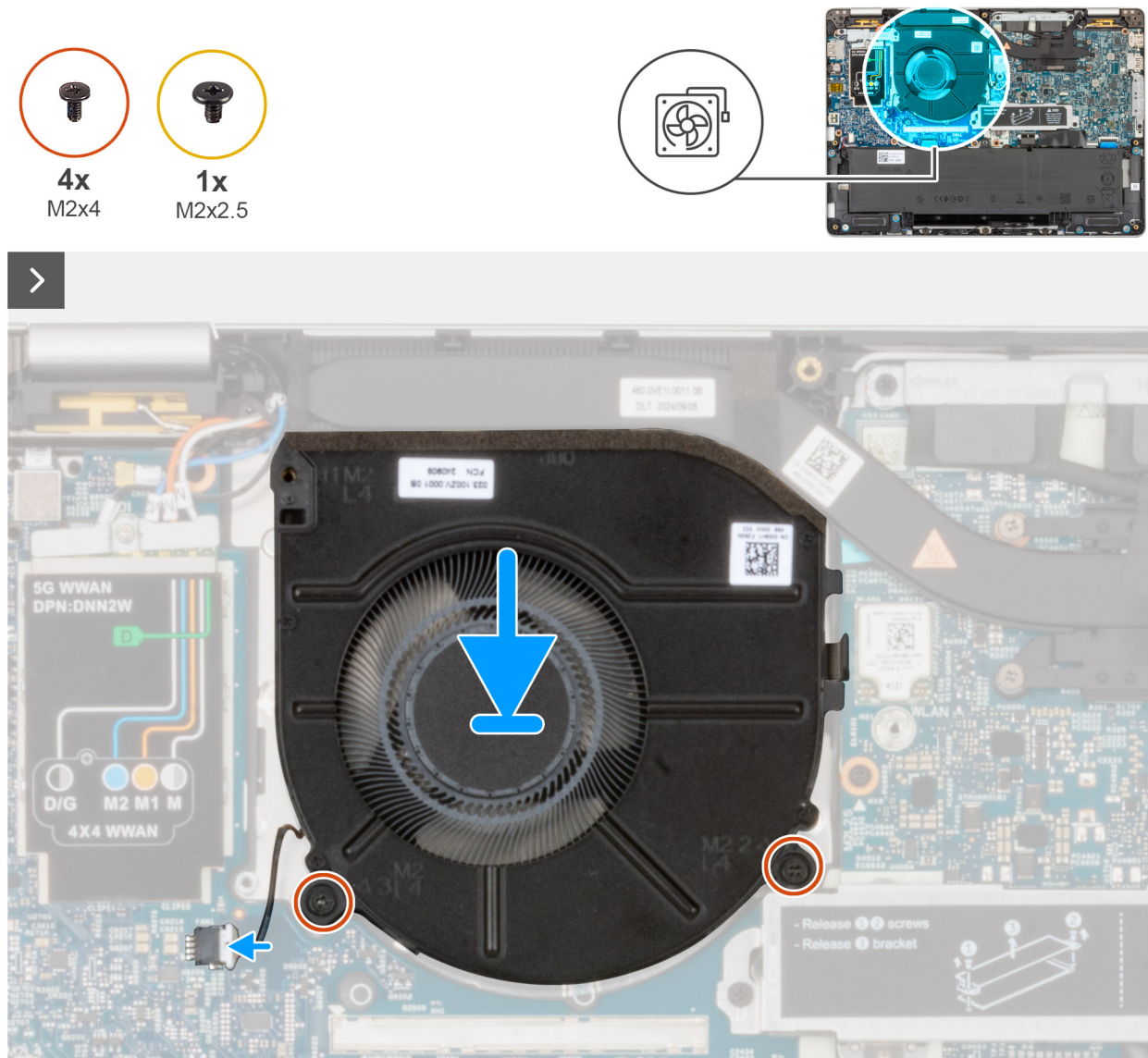
Figure 34. Installing the fan
