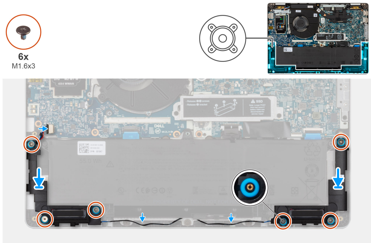
Figure 28. Installing the speakers
