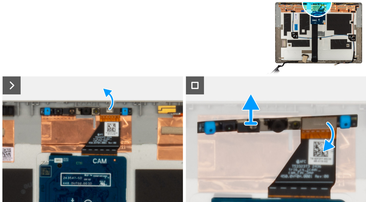
Figure 67. Removing the camera module
