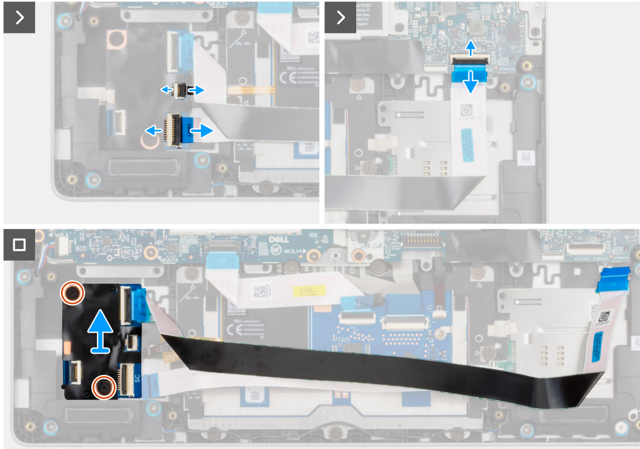
Figure 36. Removing the USH-daughter board
