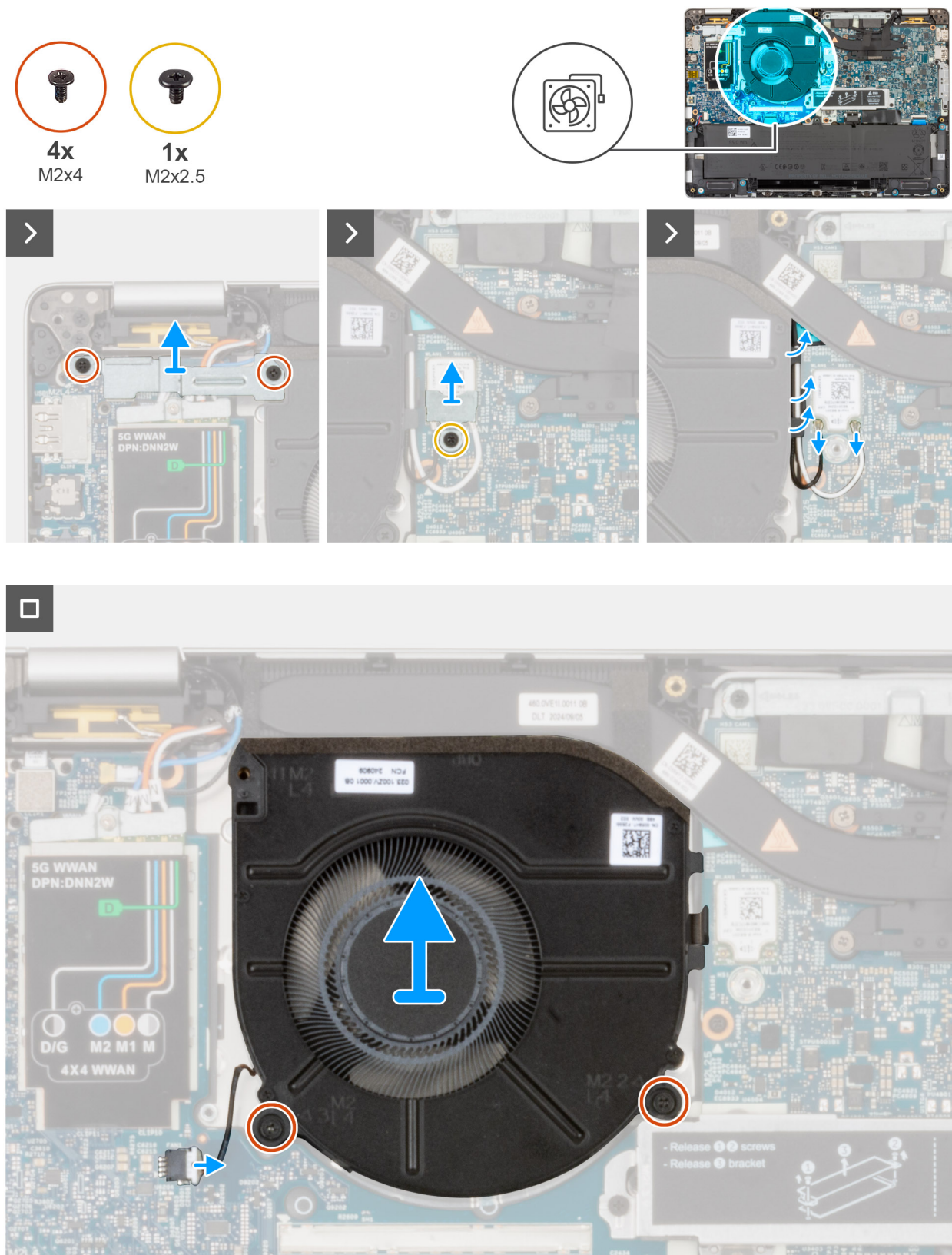
Figure 33. Removing the fan
