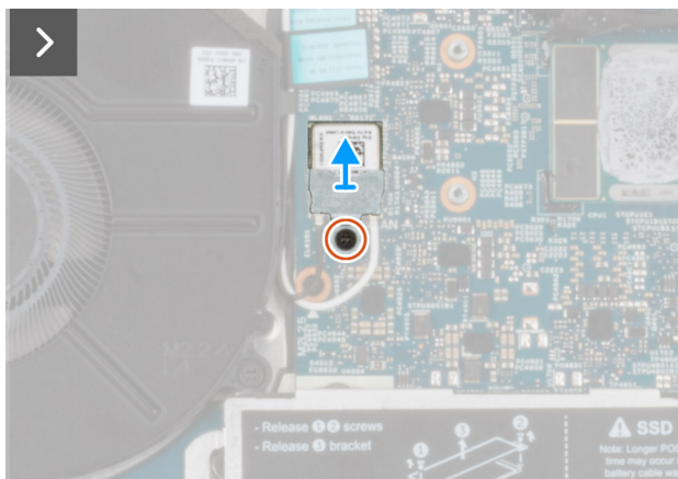
Figure 29. Removing the WLAN antenna module
