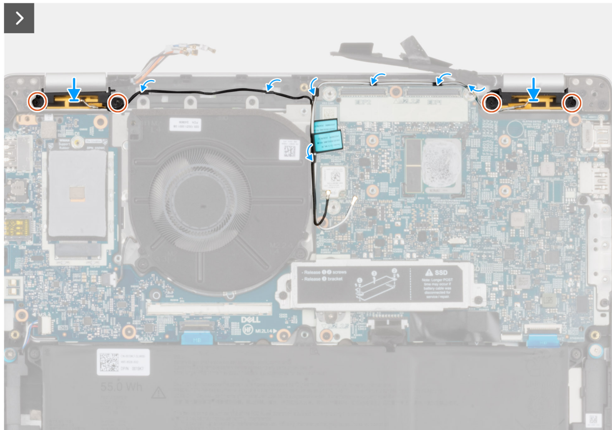
Figure 31. Installing the WLAN antenna module
