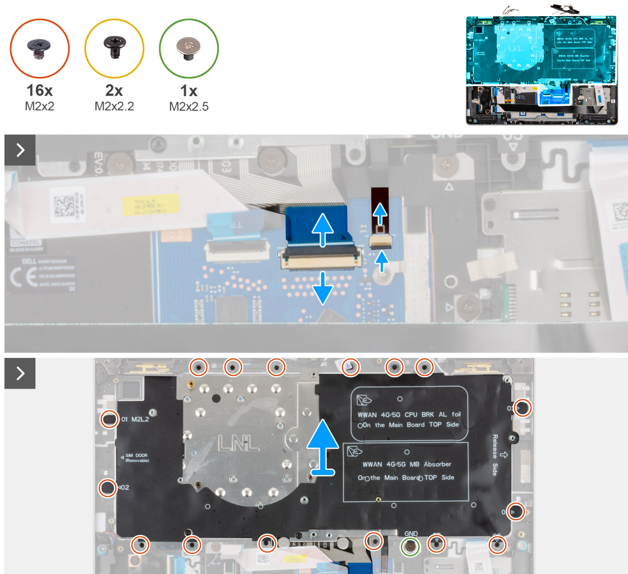
Figure 53. Removing the keyboard
