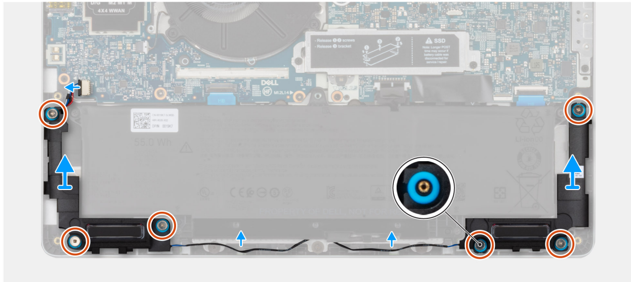
Figure 27. Removing the speakers
