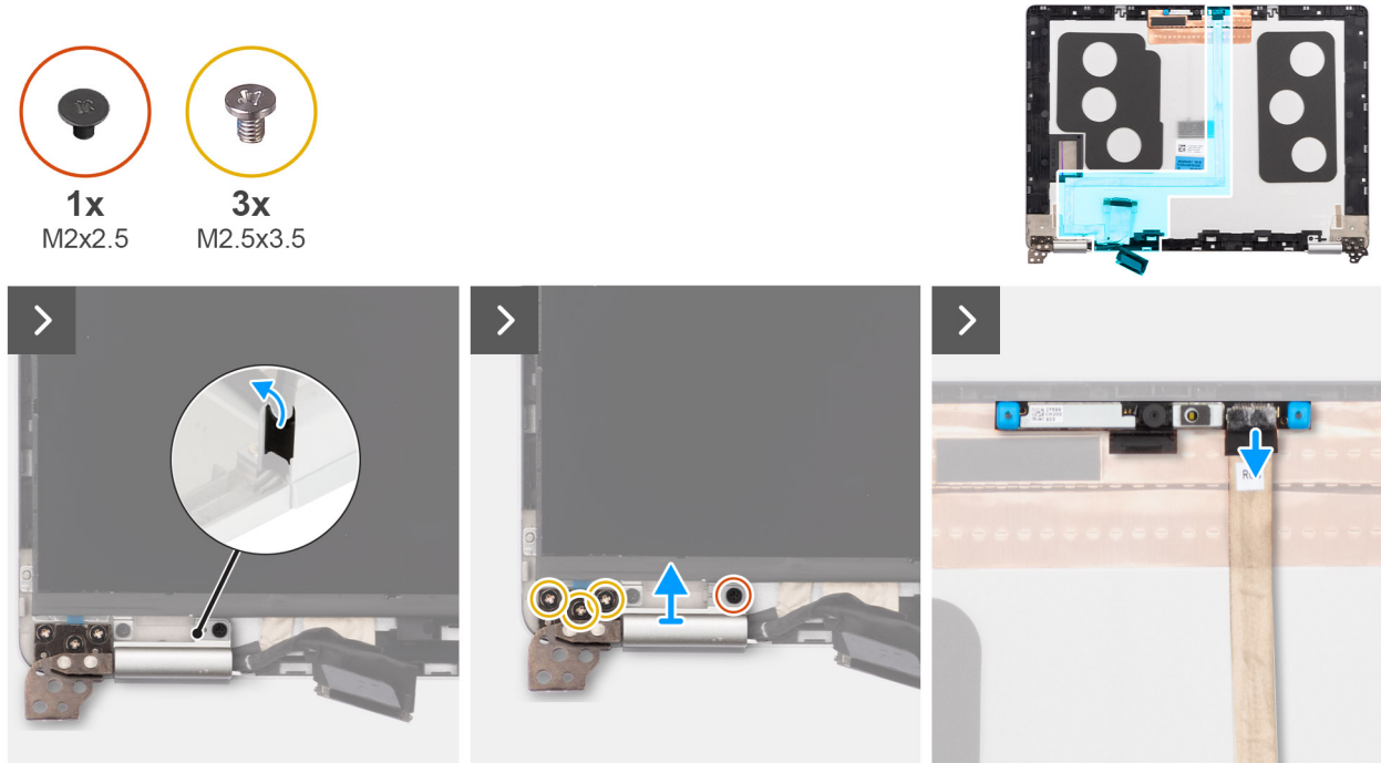
Figure 69. Removing the display cable
