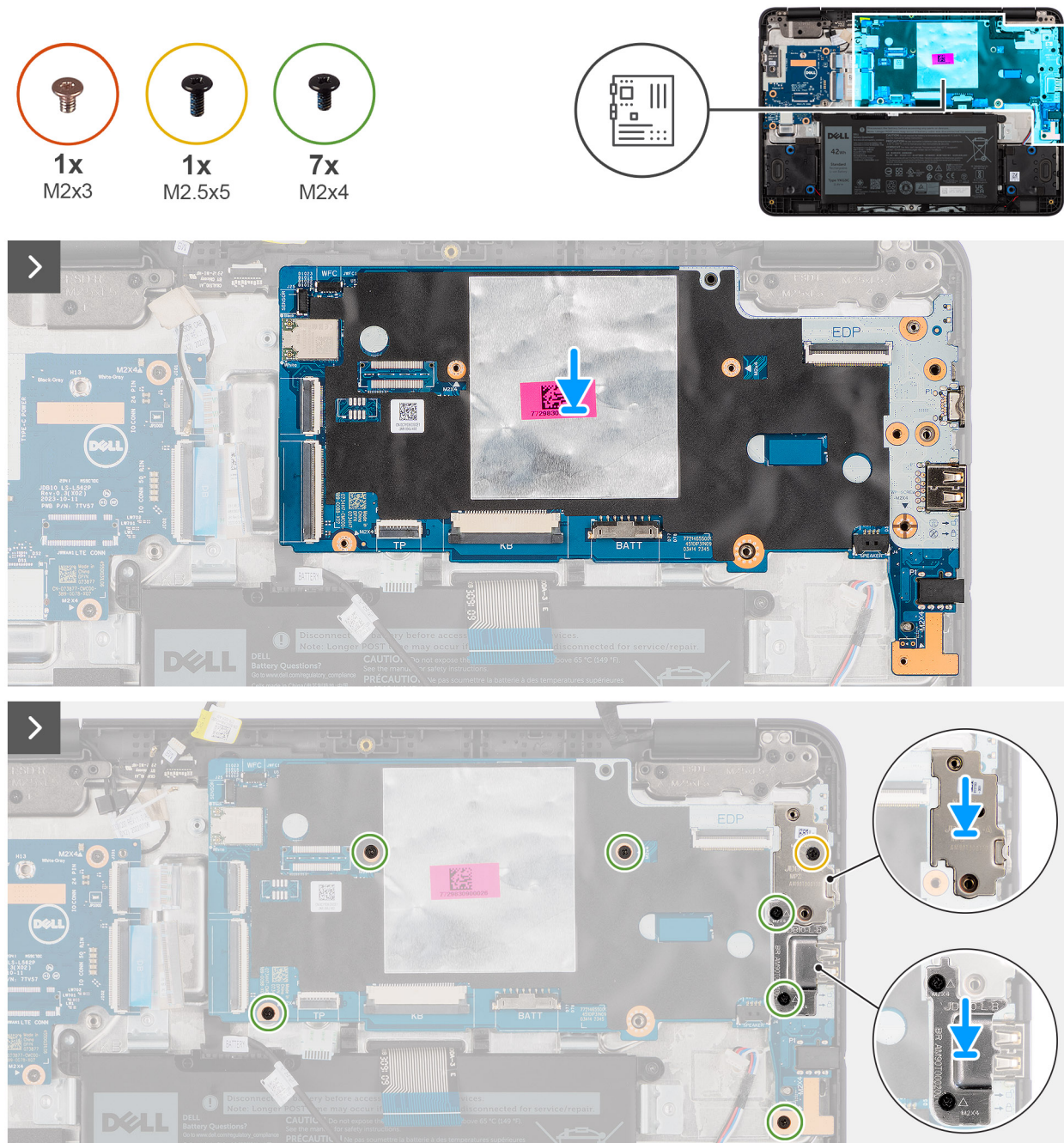
Figure 43. Installing the system board
