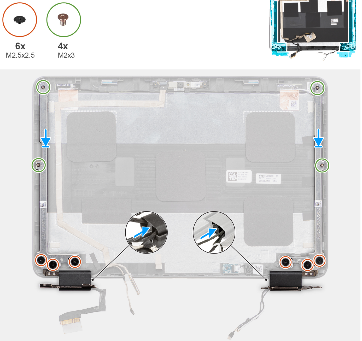
Figure 62. Installing the display hinges
