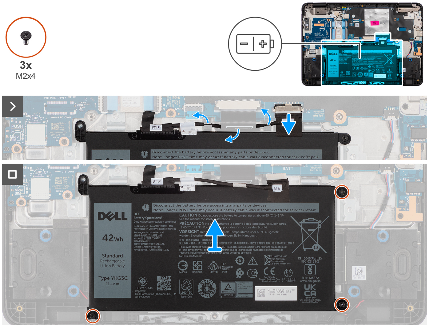
Figure 18. Removing the battery
