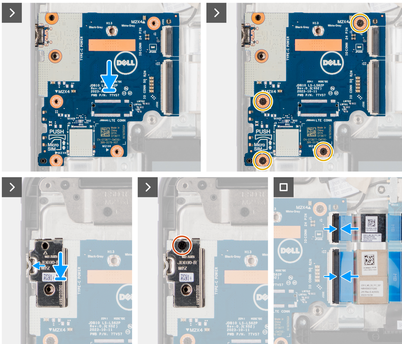
Figure 30. Installing the I/O board
