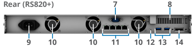
Rear (RS820RP+)
