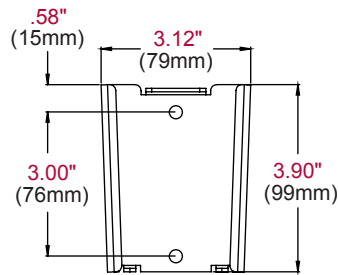
WALL PLATE
