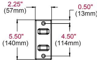
WALL PLATE
