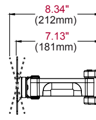
SIDE VIEW EXTENDED +/- 15° TILT
