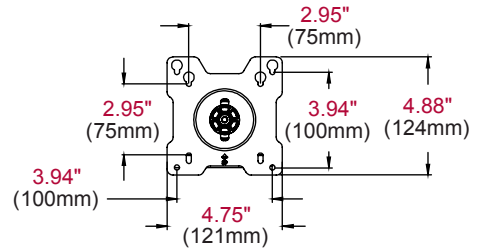
ADAPTER PLATE
